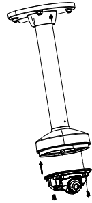
Figure 2-13 Fix the Dome Drive
