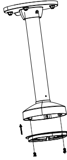
Figure 2-12 Fix the Adapter Plate
