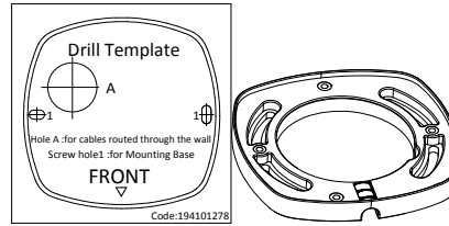
Figure 2-2 Type II Drill Template
