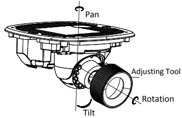
Figure 2-7 3-Axis Adjustment
