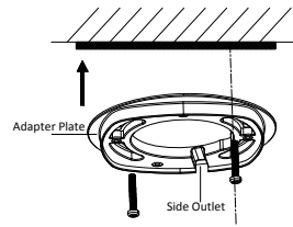
Figure 2-4 Fix the Adapter Plate
