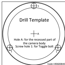
Figure 2-8 Drill Template
