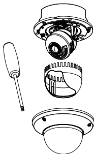
Figure 2-3 disassembling
