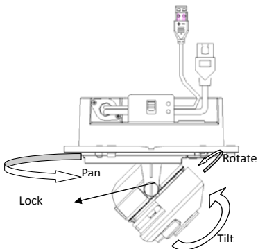
Figure 2-18 Angle Adjusting
