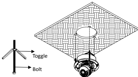
Figure 2-10 Dome Drive Installing
