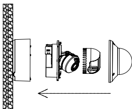
Figure 2-19 Complete the Installation
