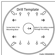
Figure 2-14 Drilling Template
