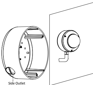
Figure 2-17 Side Cable Routing
