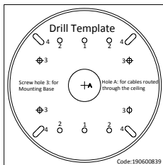
Figure 2-1 Drilling Template
