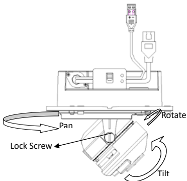
Figure 2-12 Angle Adjusting
