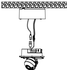
Figure 2-4 Dome Drive Installing
