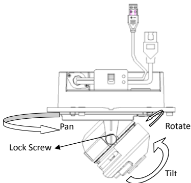
Figure 2-6 Angle Adjusting
