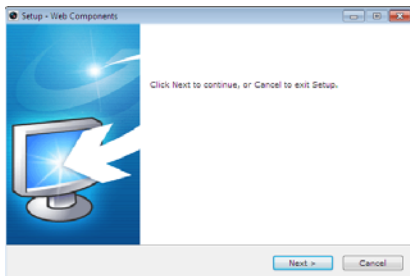
Figure 4-3 Install Plug-in (1)
