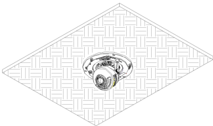
Figure 2-11 Fasten Toggle Bolt
